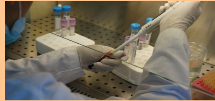
Blood Analysis
