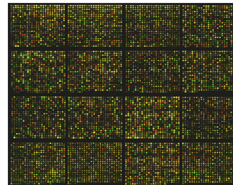
DNA Microarrays
