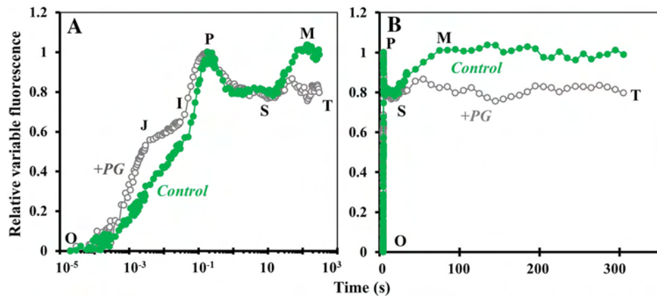
Fig. 4 (A) Chl a fluorescence transient (OJIPSMT) in wild type C. reinhardtii cells (Control) and those that had been for 10 min in darkness, with 1 mM n -propyl gallate (propyl 3,4,5-trihydroxybenzoate) (+PG)—plotted on logarithmic time scale; and (B) the same
