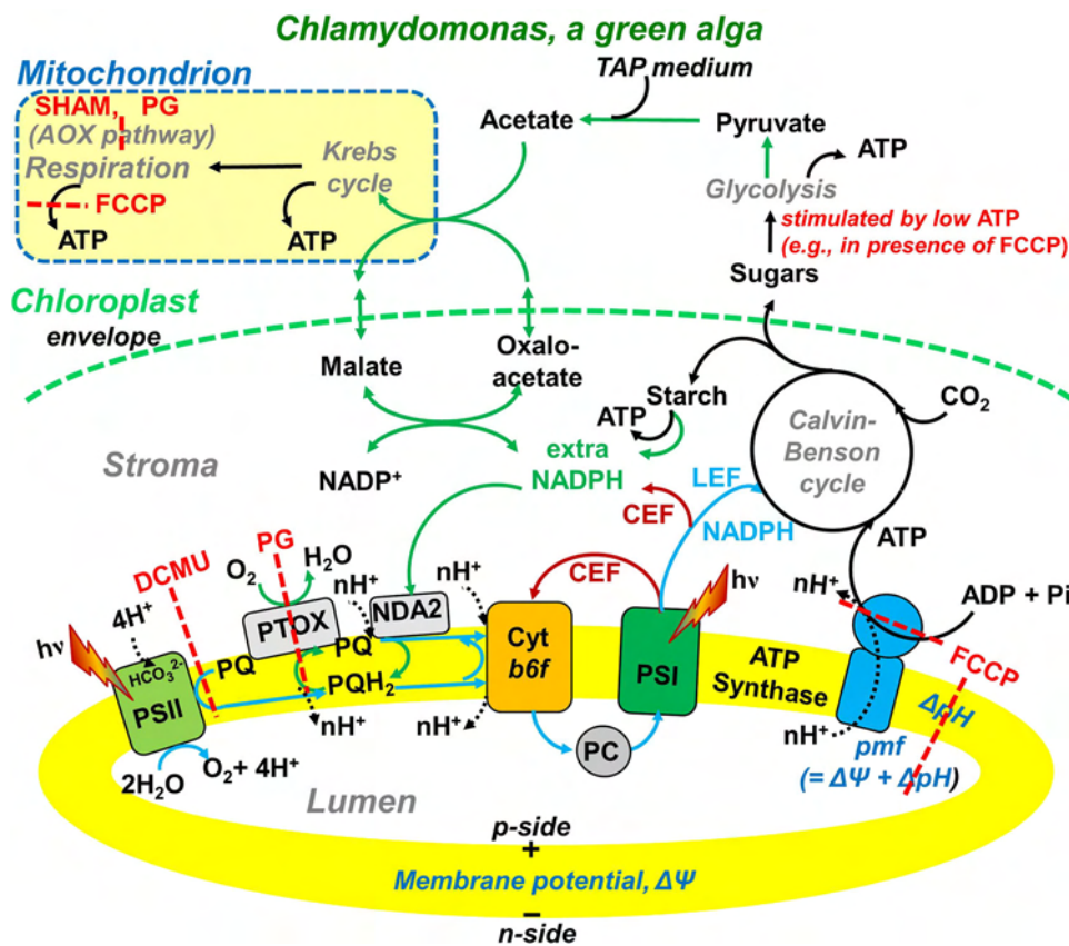
Fig. 1 A schematic representation of the interactions between electron transfer flows and carbon assimilation in the chloroplast of C. reinhardtii and metabolic reactions driven by mitochondria. Chemicals used in this study for different treatments of the algal cells are shown close to the processes affected by them. See the main text for explanation. AOX, alternative oxidase; CEF, cyclic electron flow; Cyt, cytochrome; DCMU, 3-(3,4-dichlorophenyl)-1,4-dimethyl urea; FCCP, carbonyl cyanide p -trifluoromethoxyphenylhydrazone; LEF, linear electron flow; NADP, nicotinamide adenine dinucleotide phosphate; NDA2, Type II NADPH dehydrogenase; PC, plastocyanin;
