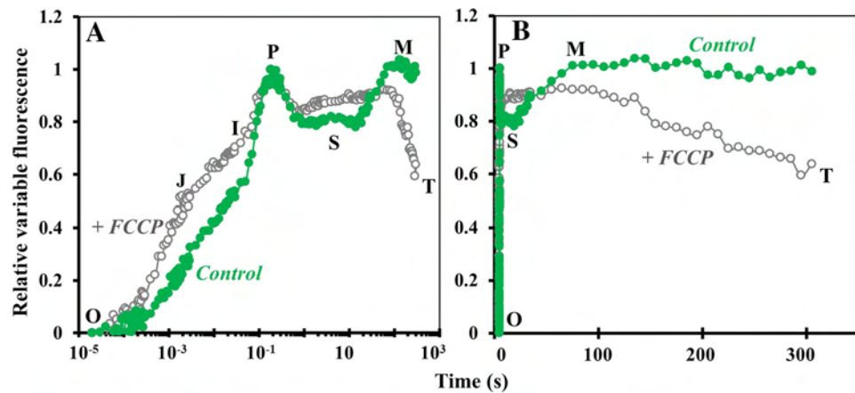
Fig. 6 (A) Chl a fluorescence transient (OJIPSM T) in wild type C. reinhardtii cells (Control) and those that had been for 10 min in darkness with 10 \mu M FCCP (carbonyl cyanide p -trifluoromethoxyphenylhydrazone) (+FCCP), plotted on logarithmic
