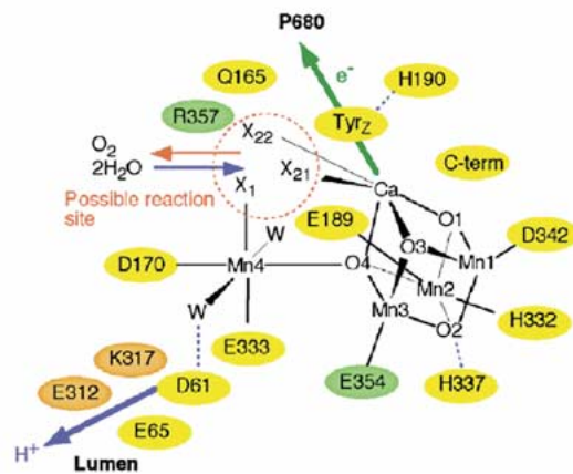
Figure 7 from J. Barber, 'Engine of life and big bang of evolution: a personal perspective,' pp. 137–155 (this issue).
