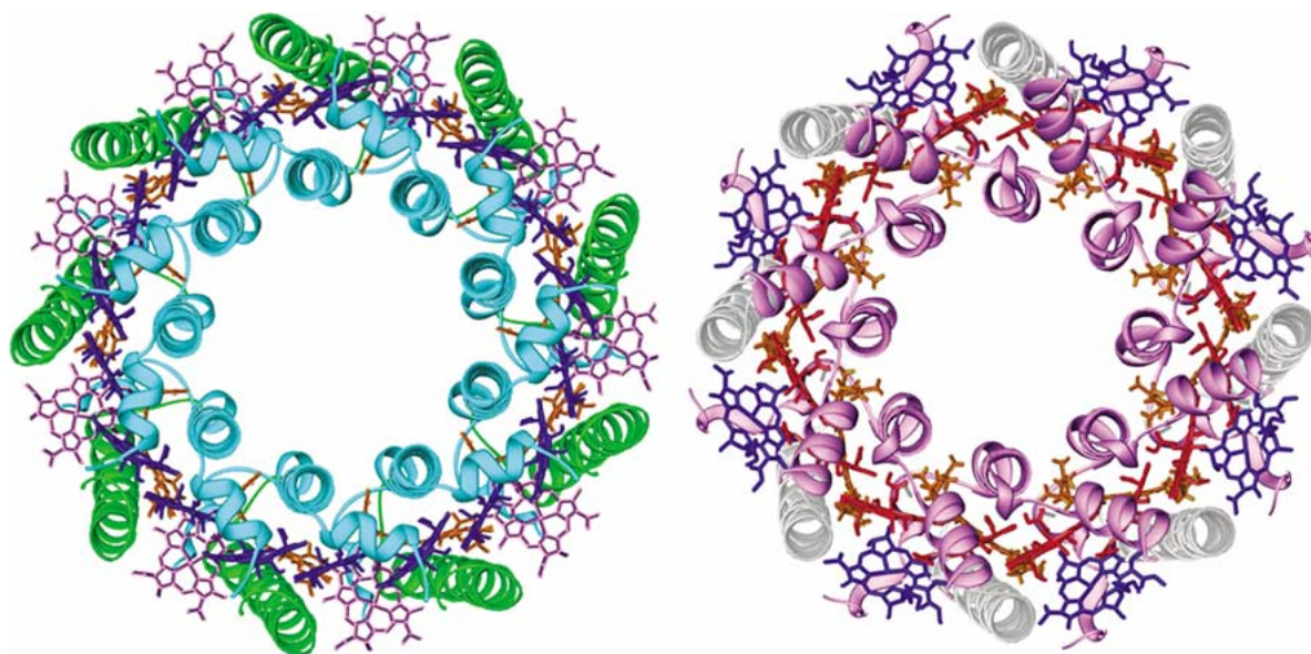
Figure 9 from R.J. Cogdell, H. Hashimoto & A.T. Gardiner, 'Purple bacterial light-harvesting complexes: from dreams to structures,' pp. 173–179 (this issue).
