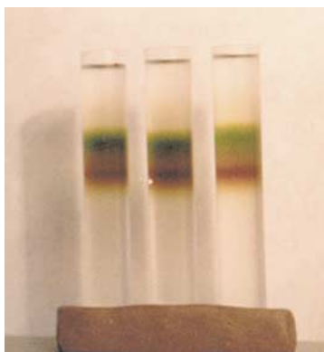
Figure 3 from G. Hauska, 'The isolation of a functional cytochrome b 6 f complex: from lucky encounter to rewarding experiences,' pp. 277–291 (this issue).
