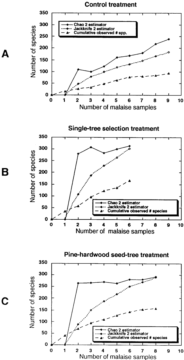
Fig. 1. Chao 2 and 2nd-order jackknife (Jackknife 2) estimator calculations of species richness in each treatment, plotted with the actual cumulative observed species found in each treatment.
