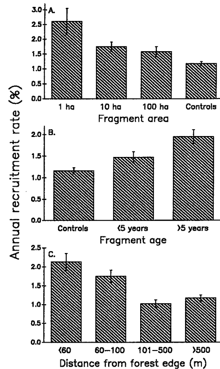
Figure 3. Effects of fragment area, age, and proximity of forest edge on annual tree recruitment rates ( \bar{X} \pm SE ).
