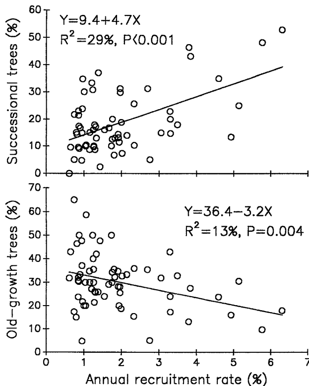
Figure 4. Relationships between annual recruitment rate and proportions of successional and old-growth tree families in study plots.
