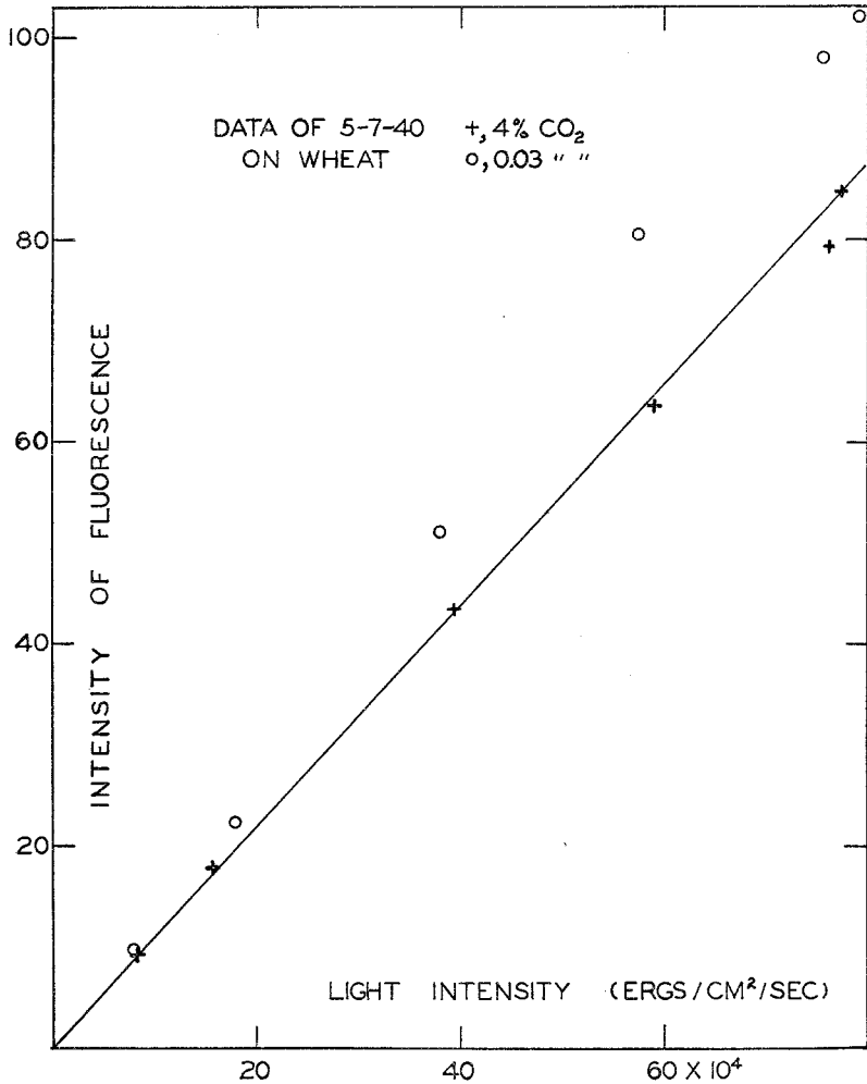
FIG. 16.—Intensity of fluorescence versus incident light intensity for wheat at 4 percent and at 0.03 percent carbon dioxide.
