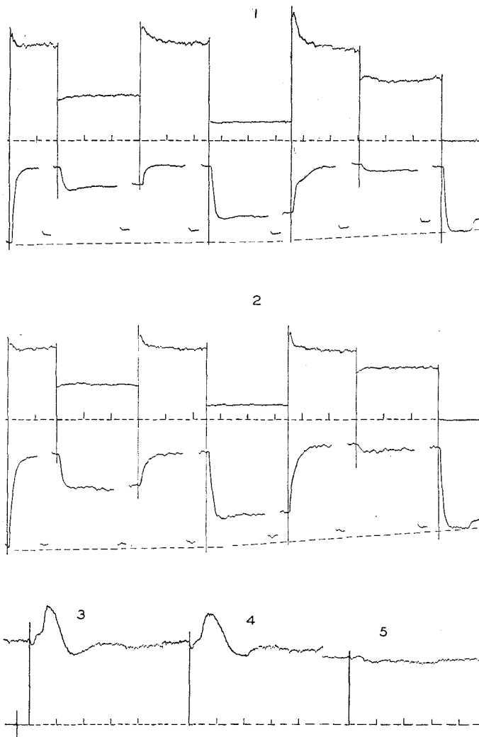
FIG. 6.—The induction behavior of wheat in response to changes in light and carbon dioxide pressure.
