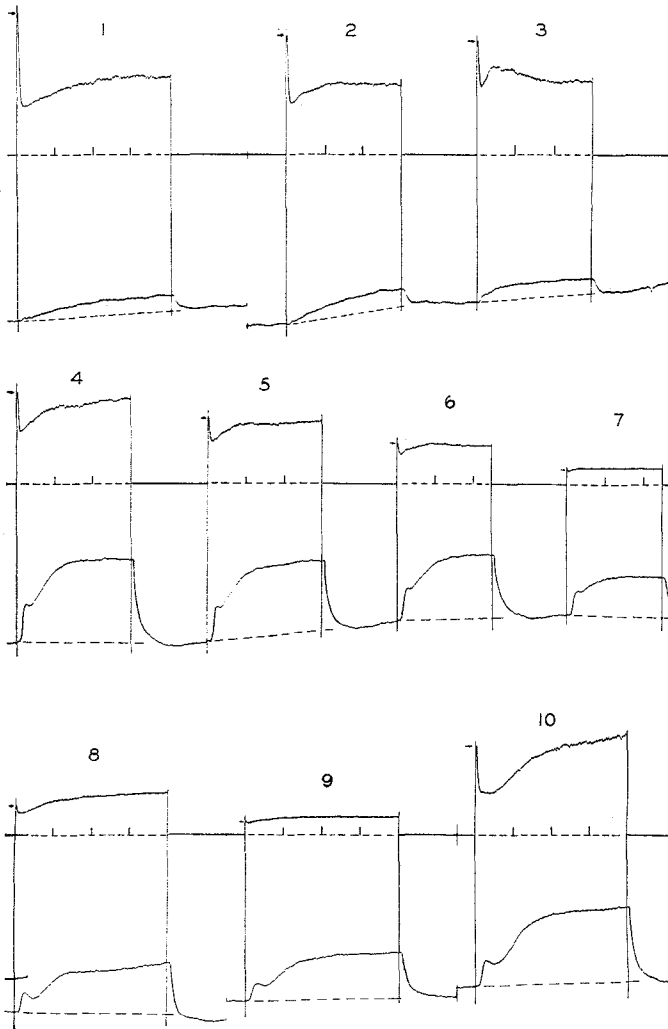
FIG. 9.—The induction behavior of Chlorella grown in air.
