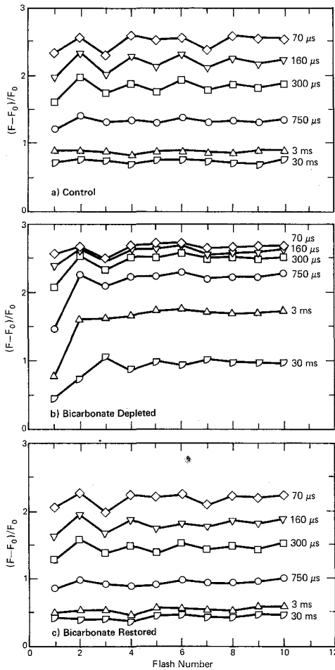
Fig. 9. The Effect of \text{HCO}_3^- -depletion, in the Presence of 25 mM \text{HCO}_2^- , on the Fluorescence Flash Pattern. The times indicated are when the measuring flash was fired. Spinach thylakoids were used; other details are as in Fig. 7 (Eaton-Rye and Govindjee, 1984, unpublished)
