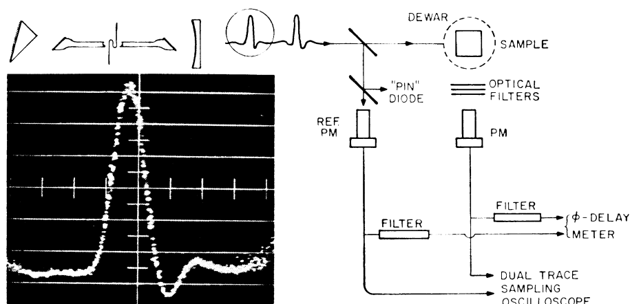
Fig. 1. Schematic of the apparatus for the measurement of fluorescence times. The inset shows a photograph of a sampling oscilloscope trace representing a mode-locked laser pulse (1 nsec/div).
