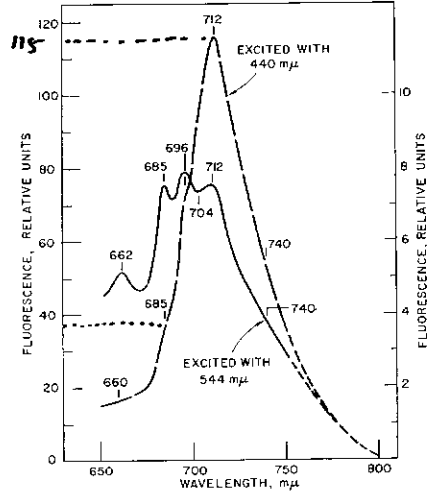
Fig. 6. Emission spectra at liquid-N 2 temperature for a 3-day-old culture of Porphyridium. Exciting wavelength: 544 mμ (solid curve, ordinate on left) and 440 mμ (long dashes, ordinate on right). Measurements beyond 750 mμ were not made and the curves have been extrapolated to zero fluorescence at 800 mμ.
