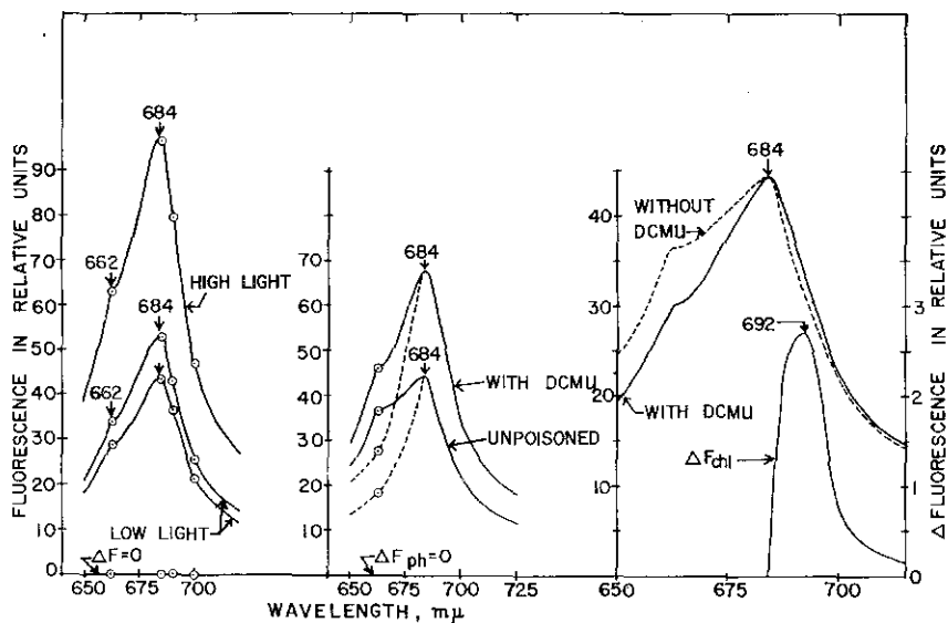
Fig. 5. Effect of DCMU on the emission spectra of Porphyridium. (a) left: Emission spectra obtained upon excitation with 544-m \mu light after addition of 50 \mu M DCMU for "low" (lower curves) and "high" (upper curve) intensity of exciting light. The \Delta F curve shows no difference in the shape of the emission spectra at "low" and "high" light intensities. (b) middle: Emission spectra for poisoned and unpoisoned cells. \Delta F_{Pn} = 0 ; no change in phycocyanin fluorescence (see text). (c) right: The emission spectra for poisoned (50 \mu M DCMU; solid curve) and unpoisoned (dashes) cells (both at "low" intensity) are normalized at the chlorophyll a peak. Exciting wavelength: 544 m \mu . The difference emission (solid curve) between poisoned and unpoisoned cells is shown on a ten times enlarged scale. \Delta F_{chl} = change in chlorophyll fluorescence. Note the peak at 692 m \mu .
