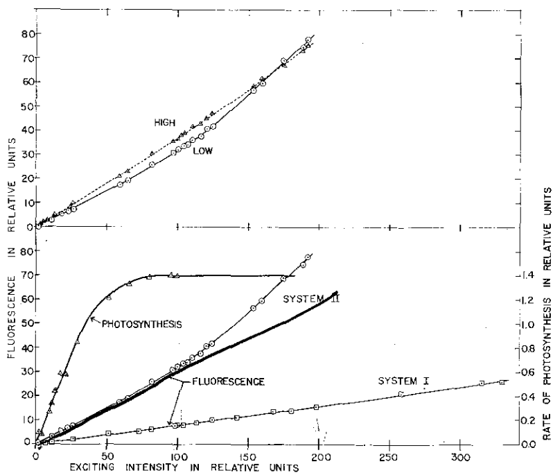
Fig. 2. Fluorescence intensity at 688\text{ m}\mu as a function of intensity of incident exciting light. 100 units on the abscissa correspond to 1.00 \cdot 10^{15} quanta \cdot \text{cm}^{-2} \cdot \text{sec}^{-1} . Top: Light curves [ F = f(I) ] for "high-light cells" (triangles) and "low-light cells" (circles) upon excitation with 544\text{-m}\mu light at room temperature. The absorbance for both types of cells was adjusted to be the same at 544\text{ m}\mu . Bottom: Light curves upon excitation in System I (blue light, squares) and System II (green light, circles) at room temperature. The curve with triangles is for the rate of photosynthesis as a function of intensity of green light obtained with only one green filter, Schott VG-5. (Photosynthesis data cannot be too accurately compared with the fluorescence data because of somewhat different spectral characteristics of exciting light used in the two cases.)
