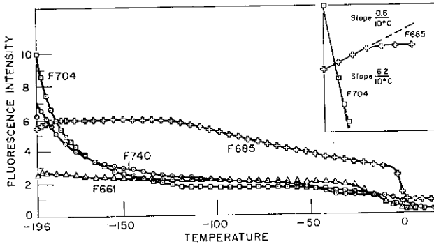
Fig. 8. Fluorescence intensity at 685\text{ m}\mu (F685), at 704\text{ m}\mu (referred to in the figure as F704; as F696 in the text), at 740\text{ m}\mu (F740; as F720 in the text) and at 661\text{ m}\mu (F661; as F660 in the text) as a function of temperature [ F = f(T) ]. Exciting light: 440\text{ m}\mu . Insert shows rate of change of fluorescence intensity at 685\text{ m}\mu and at 704\text{ m}\mu between -196^\circ and -185^\circ (both scales for the insert are on a three times expanded scale).
