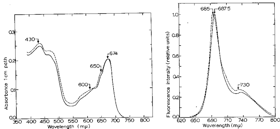
Fig. 1. Absorption spectra of deuterated (---) and hydrogen (—) C. vulgaris . The numbers on the graph show the location of certain points in m \mu . The curves have been adjusted to give the same absorbance at 674 m \mu .
